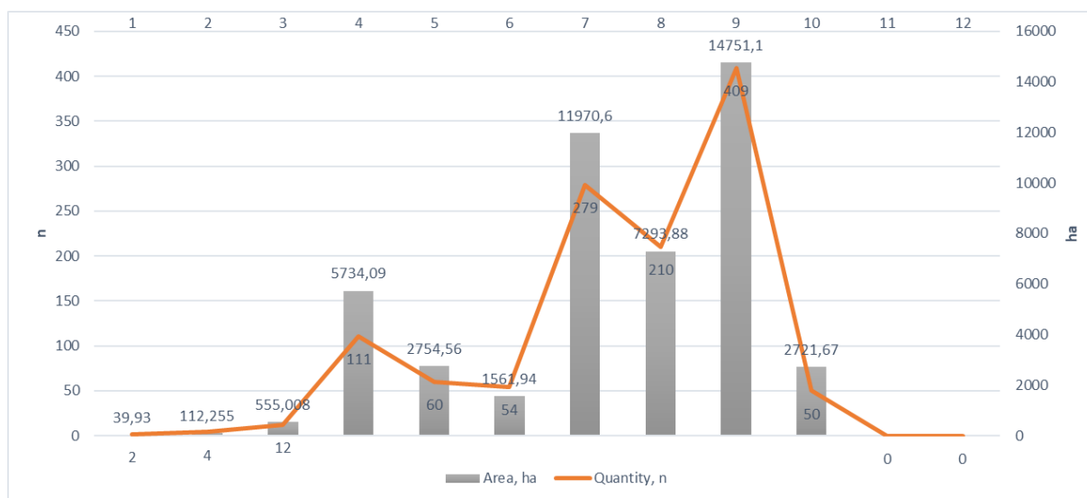
Fig. 1. Monthly Dynamics of Fire Incidents and Burned Area in 2025
